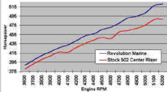
Revolution Marine Exhaust Horsepower Comparison
